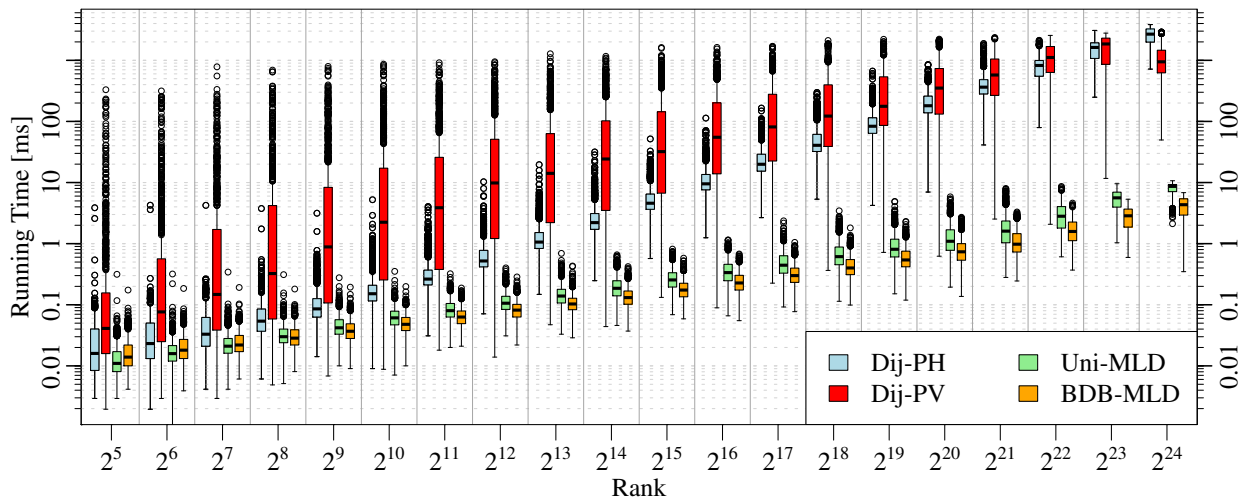
Figure 2: Running times subject to Dijkstra rank for our algorithms on the Europe EV-1000 instance. Smaller ranks indicate more local queries. Reachability flags for the MLD algorithms are disabled and battery capacity is increased to the point where it does not constrain vehicle range.
