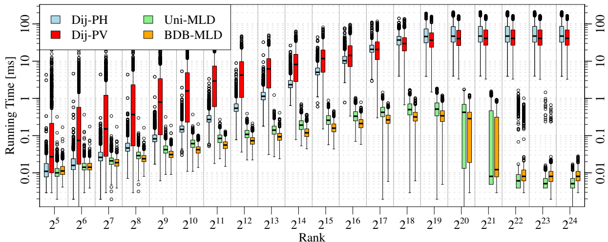
Figure 3: Running times subject to Dijkstra rank for our algorithms on the Europe PG-16 instance. We enable reachability flags for the MLD algorithms. As in Figure 2, smaller ranks indicate more local queries.
