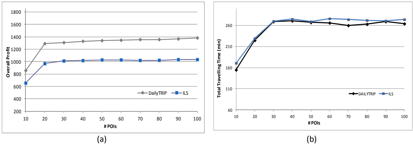
Figure 5. (a) Comparison of the overall profit of DailyTRIP vs ILS for 2 itineraries; (b) comparison of the total travel time derived from DailyTRIP and ILS for 3 Itineraries.
