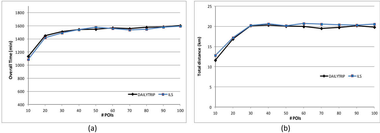
Figure 6. (a) Comparison of the overall time derived from DailyTRIP and ILS algorithms for 3 itineraries; (b) comparison of the total distance for 3 itineraries.
