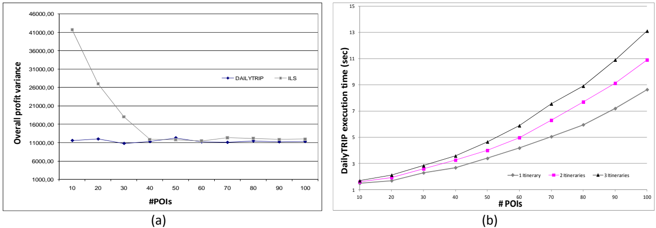
Figure 7. (a) Variance of the individual itineraries' overall profit per day for both algorithms (4 daily itineraries); (b) execution time of DailyTRIP for a varying number of POIs and itineraries.
